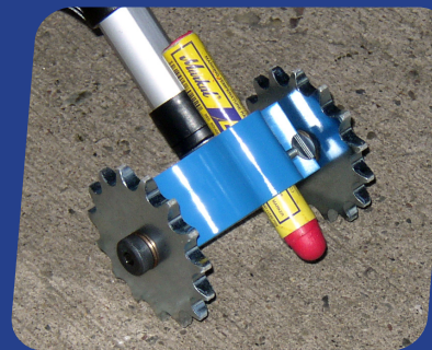
Delamination Detection Tool shown with attached crayon for on-the-spot marking of delaminated areas.
